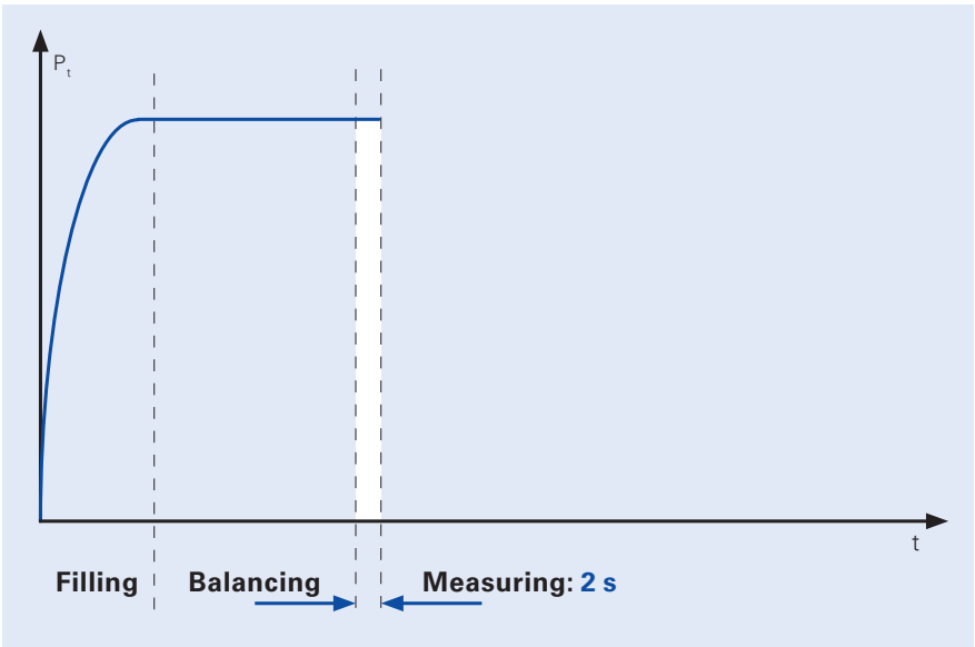
Duration of the measuring phase for leak test on an oil chamber (typical test volume: 25 l)
